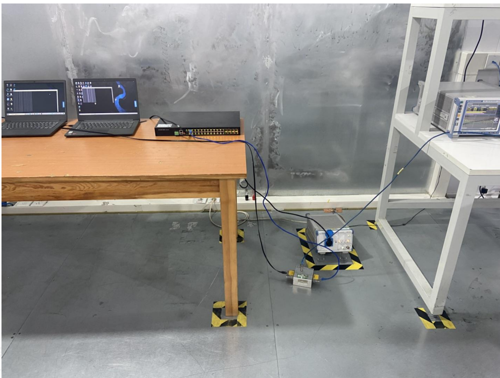
Test Setup Photo of Telecommunication Line Conducted Emission Measurement
