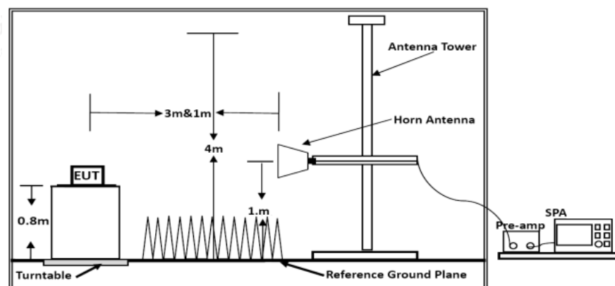
Above 1GHz
