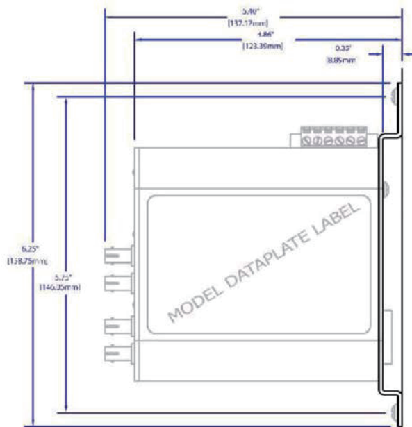
OPTIONAL COMPACT PANEL MOUNT ASSY. ( P/N: CPMA-2 )
